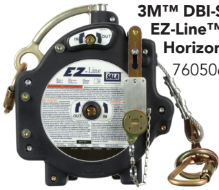
3M™ DBI-SALA® Horizontal Lifeline Cable Assembly, Single Span, 60 ft
